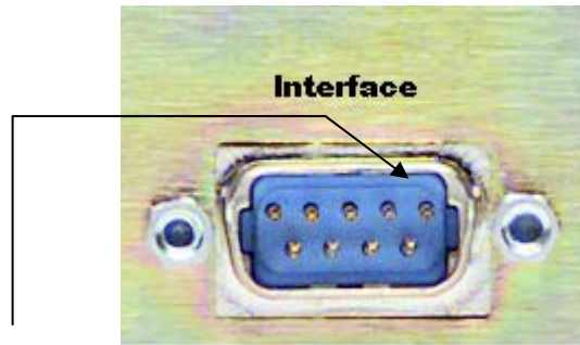
Pin 1 Rear Panel Interface Connector for Remote Trigger Script Activation
