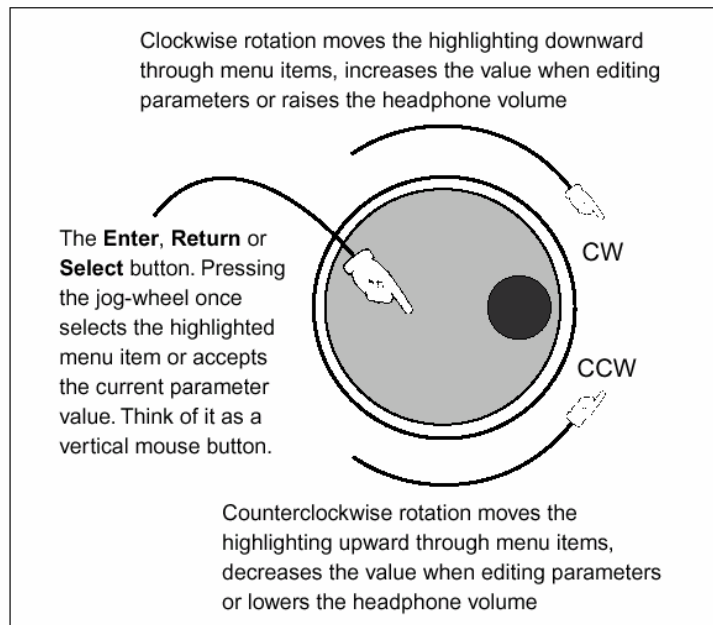
Jog-Wheel Functions
